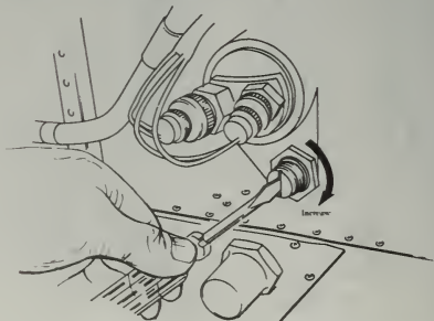
FIGURE 6-21. Oil pressure relief valve adjustment.
